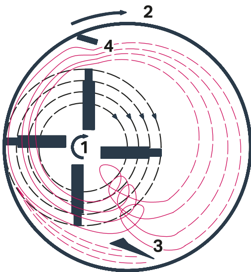
Mixing process
